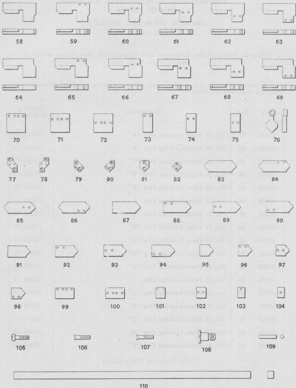
LOCKING DOGS AND DETAILS FOR STYLE "A" INTERLOCKING MACHINE
